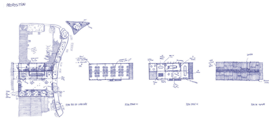
Fig. 6 - Proposed plans of the intervention in Fig. 4.
